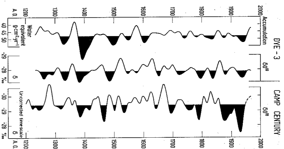
Fig. 11. Digital-filter smoothed records of annual accumulation at Dye 3 (left \delta(\text{O}^{18}) ) at Dye 3 and Camp Century. The Dye 3 data (including the time scale) are based on a continuous series of 740 seasonal \delta oscillations. The Camp Century scale is based on the assumption of unchanged accumulation rate. This is the reason why the two \delta curves are occasionally out of phase. However, both show the climatic optimum around 1930, and generally sub-normal \delta 's during "the little ice age". Some correlation (coefficient 0.6) appears between accumulation and \delta curves from Dye 3, sub-normal accumulation occurring in periods.
