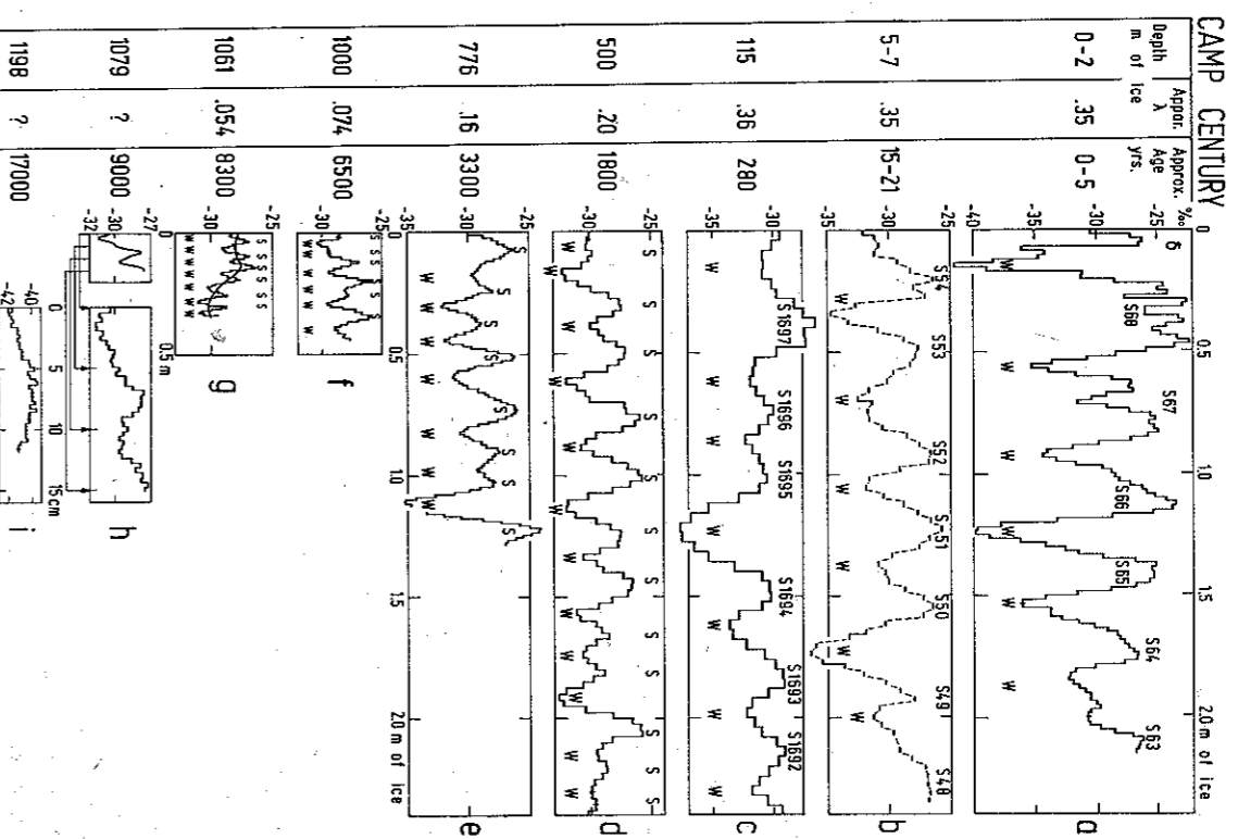
Fig. 6. (From JOHNSON et al. , 1972). The \delta oscillations in firn and in ice cores from the depths below surface indicated to the left of the figure at Camp Century. S and W indicate interpretations of summer and winter layers, respectively. As the ice sinks towards the bottom, thickness, \lambda , of the annual layers is reduced due to plastic deformation. Within a few years (a and b) short-term \delta variations are obliterated by mass exchange in the porous firn. After some decades (b and c) the seasonal \delta amplitude is reduced to about 2\text{‰} . Further reduction takes place only by molecular diffusion in the solid ice and becomes effective only when, after thousands of years, the thinning of the layers has increased the \delta gradients considerably (d to i).
